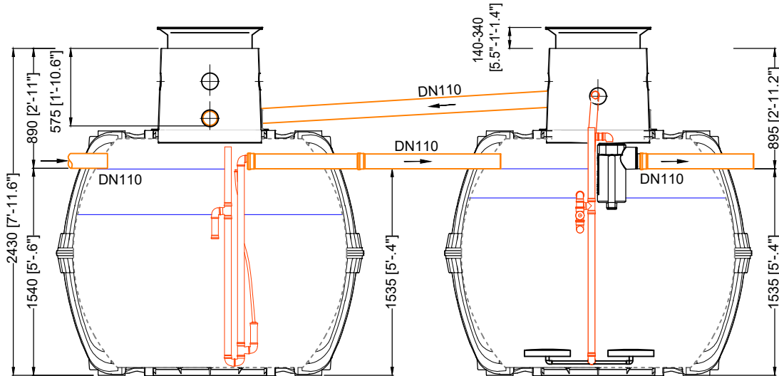
Schlamm-speicher/ Puffer sludge storage/ buffer
