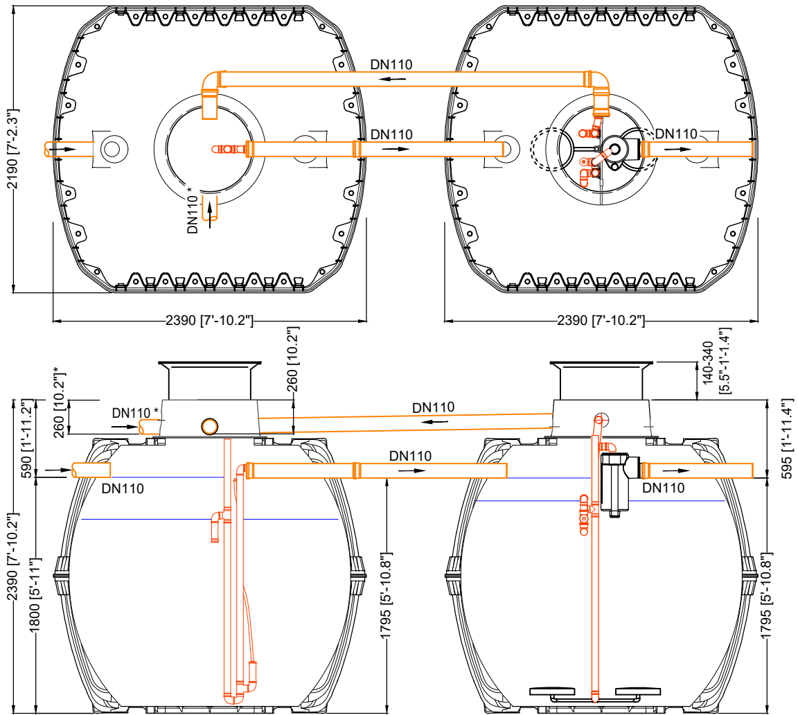
Schlamm Speicher/ Puffer sludge storage/ buffer
