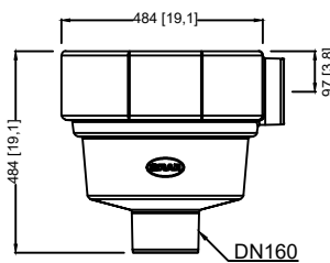
Pedestrian Loading Lid (Maxi)
